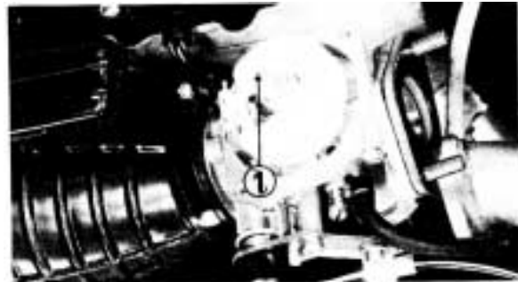
(1) Main jet
