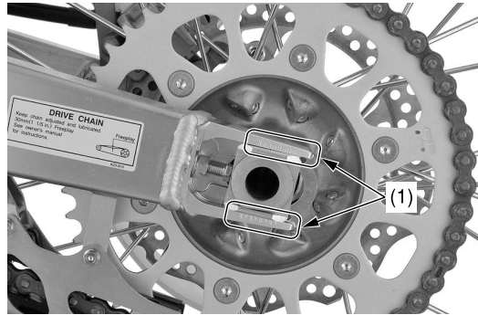
(1) chain adjuster index marks
