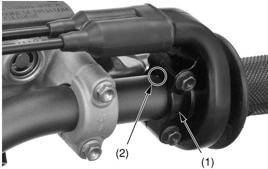
(1) throttle housing (2) paint mark
