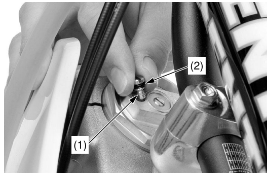
(1) pressure release screw (2) O-rings
