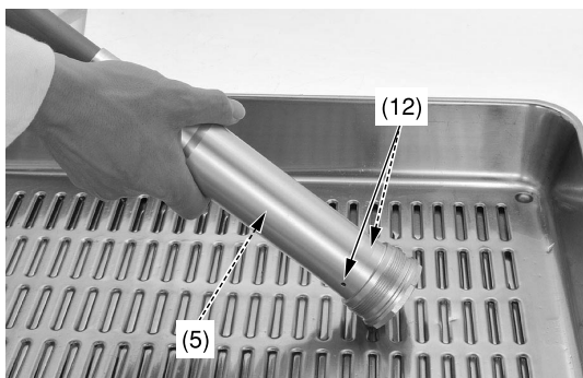
(5) fork damper oil chamber (12) oil holes
