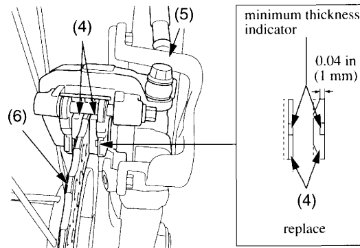
(4) brake pads (5) rear brake caliper (6) brake disc
