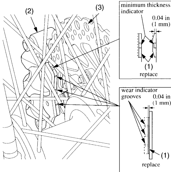
(1) brake pads (2) front brake caliper (3) brake disc
