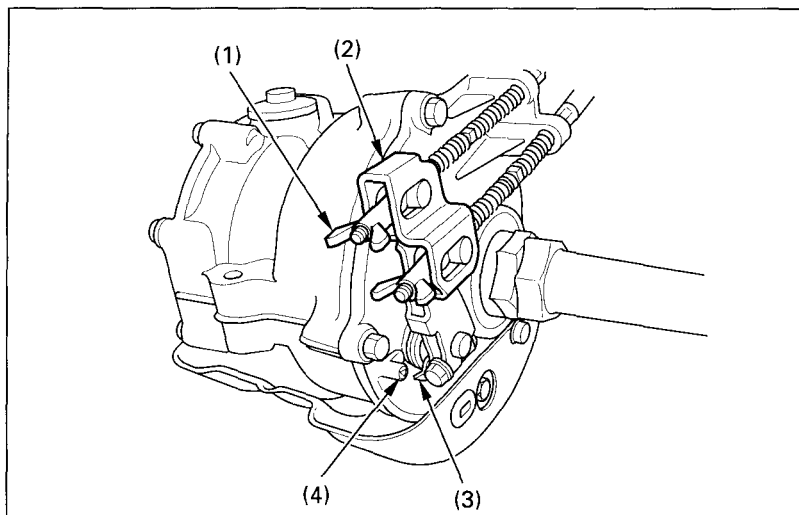
Fig. 4-25 (1) Brake lever adjusting nut (2) Brake arm (3) Arrow (4) Reference mark
