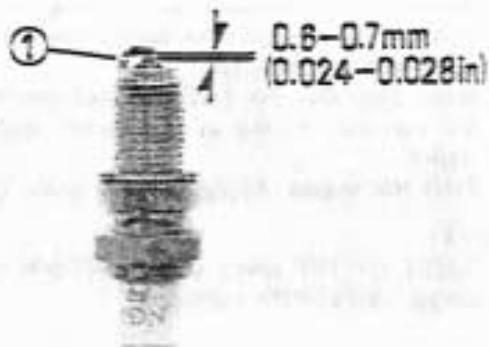
(1) Side electrode
