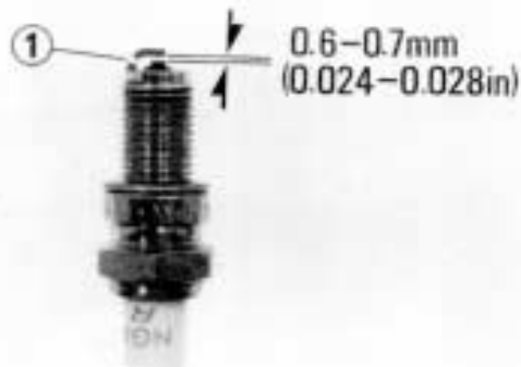
(1) Side electrode
