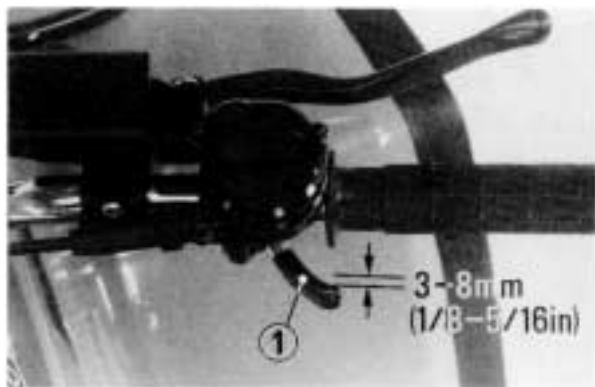
(1) Throttle lever
