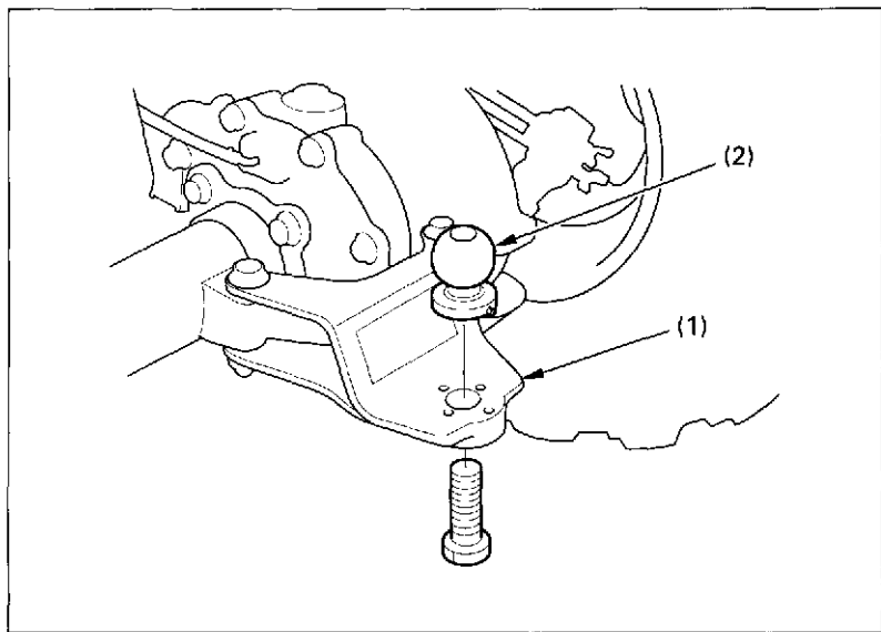
Fig. 2-24 (1) Trailer hitch
