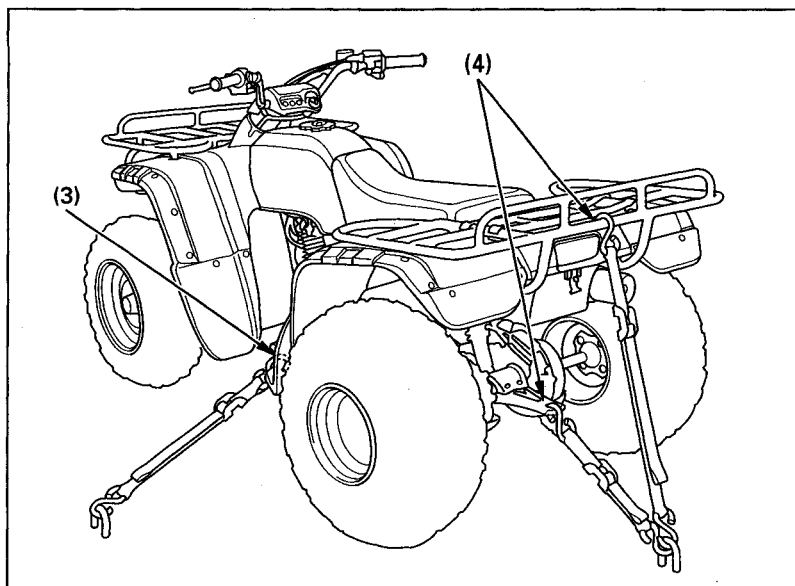
Fig. 4-38 Points to secure FOURTRAX with tie downs
