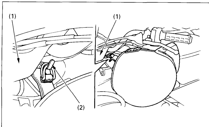
Fig. 2-20 (1) Handlebar cover
