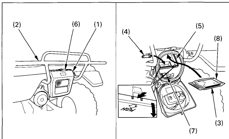
Fig. 2-30 (1) Storage compartment
