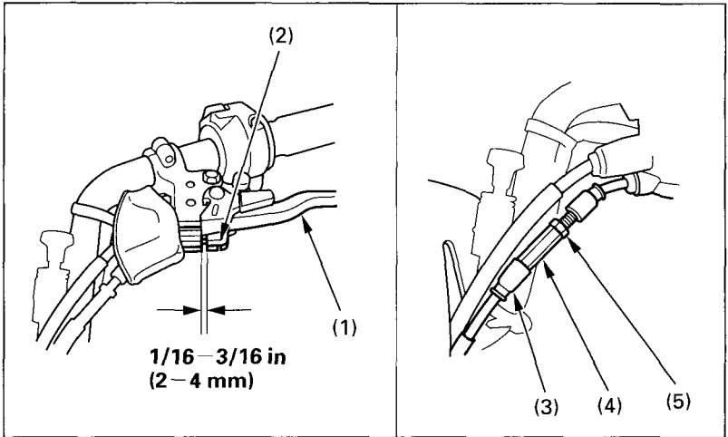
Fig. 4-18 (1) Rear brake lever (2) Reverse assist lever
