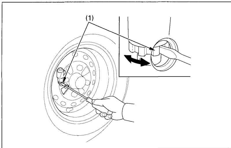
(1) Brake adjusters
