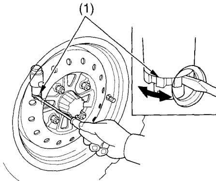
(1) brake shoe adjuster
