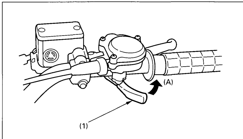
Fig. 2-11 (1) Throttle lever
