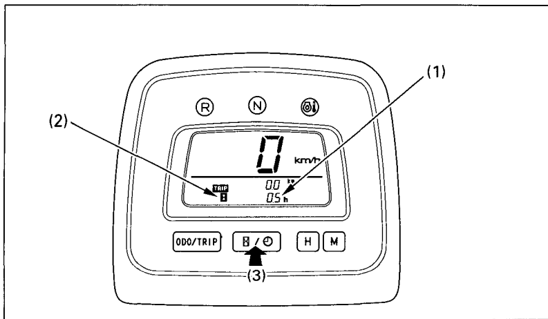
(3) Hourmeter/digital clock select button
