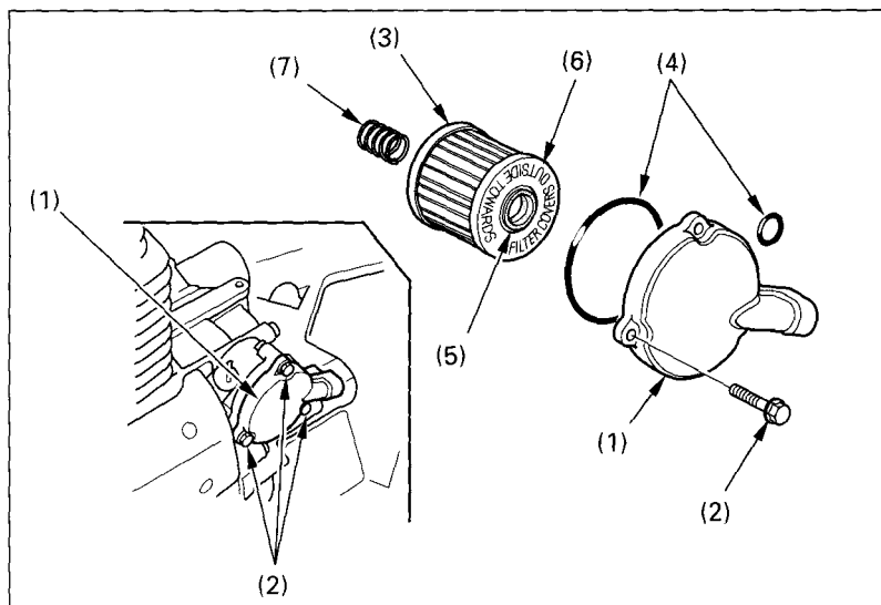
Fig. 4-12 (1) Oil filter cover (2) Bolts (3) Oil filter (4) O-rings
