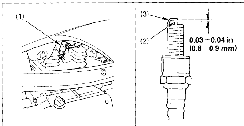
Fig. 4-14 (1) Spark plug cap
