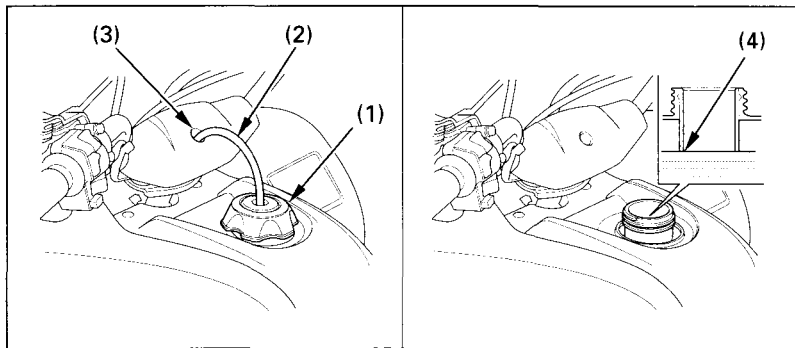
Fig. 4-2 (1) Fuel fill cap (2) Breather tube (3) Handle cover hole
