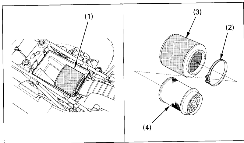
(3) Air cleaner (4) Air cleaner body
