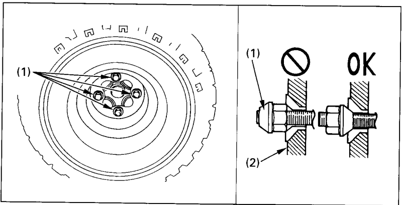
Fig. 4-30 (1) Wheel nuts
