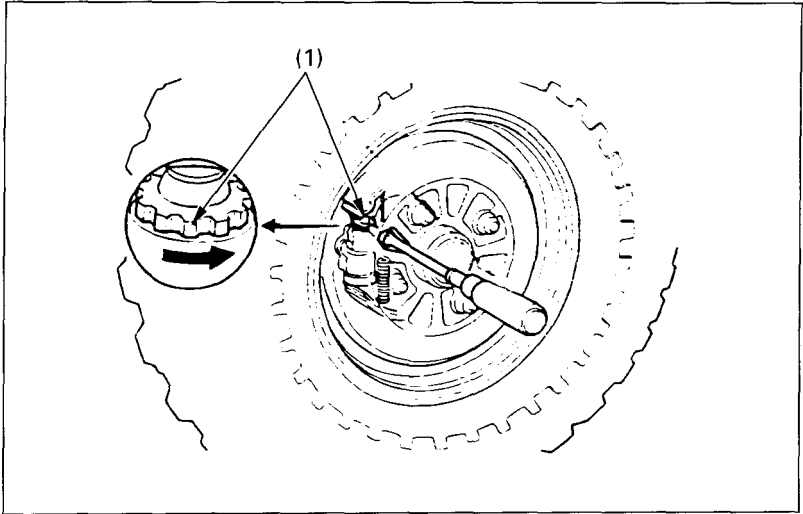
(1) Brake adjusters
