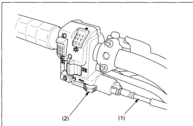
Fig. 4-8 (1) Choke cable
