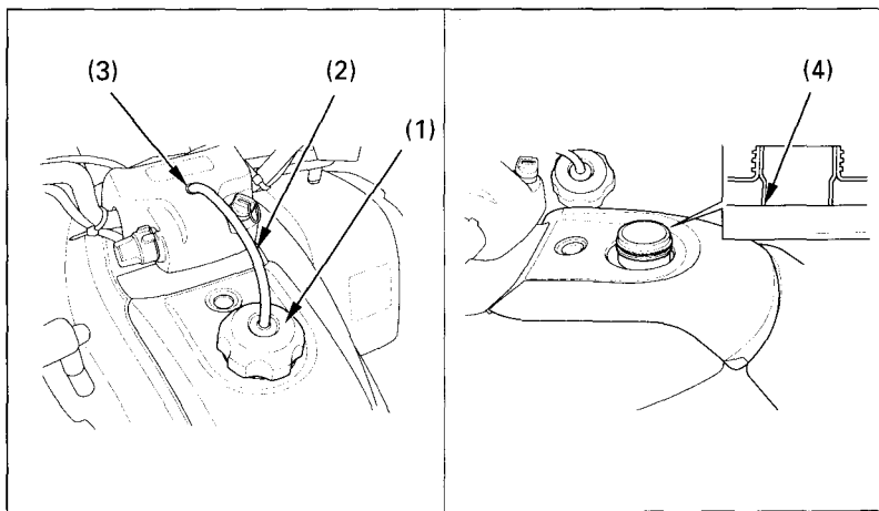
Fig. 4-3 (1) Fuel fill cap (2) Breather tube (3) Handlebar cover hole
