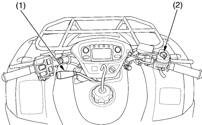
(1) gearshift lever
