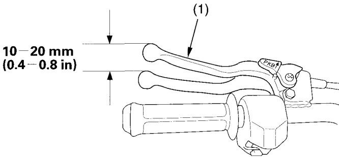
(1) rear brake lever
