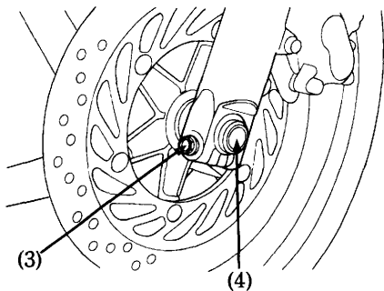
(3) Axle pinch bolts (4) Front axle
