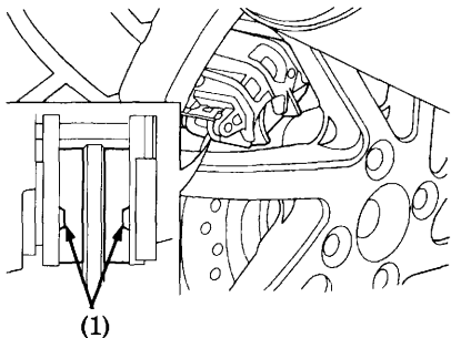
(1) Cutouts
