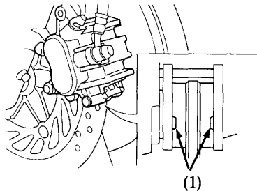
(1) Cutouts
