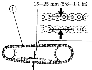
(1) Drive chain
